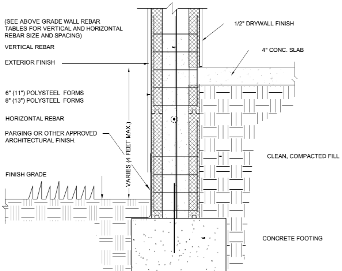
FIGURE 3.23 STEM WALL AND INTEGRATED SLAB FOR POLYSTEEL WALL CONSTRUCTION
