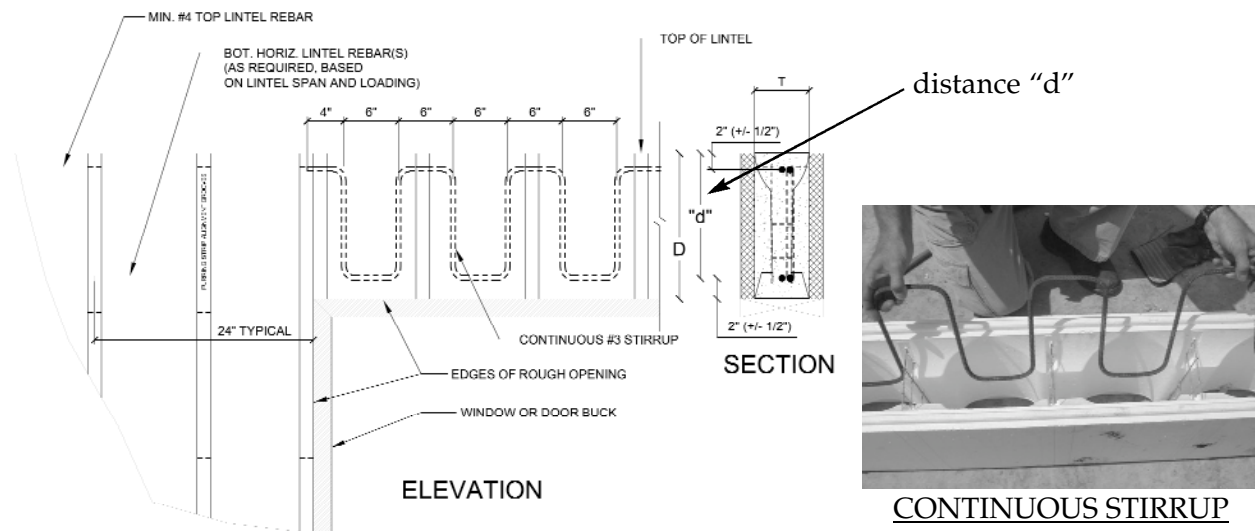
FIGURE 4.5 CONTINUOUS STIRRUP
